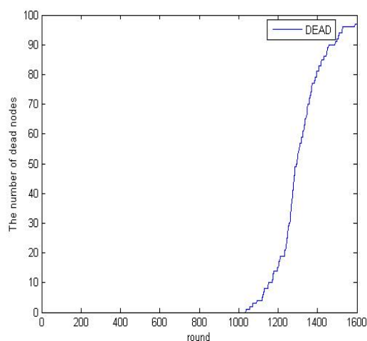
Figure 10. The dead nodes using rough sets per round with 100 nodes
